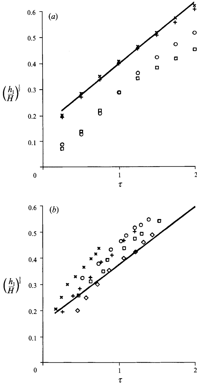
FIGURE 3. A plot of (h_1/H)^{\frac{1}{2}} , where h_1 is the distance of penetration of lower-layer fluid into the upper layer, non-dimensionalized by the depth H of the tank, against the dimensionless time \tau . (a) The numerical calculations for 90^\circ mesh and 180^\circ mesh, respectively, with (+, x) and without (O, □) the long-wave perturbation. The solid line is the best fit straight line to the 180^\circ mesh data with the long-wave perturbation. (b) The experimental results for a range of Atwood numbers: x, A = 3.3 \times 10^{-3} ; +, A = 9.5 \times 10^{-3} ; O, A = 2.2 \times 10^{-2} ; □, A = 3.2 \times 10^{-2} ; ◇, A = 4.3 \times 10^{-2} . The solid line is the same line as plotted in (a).
