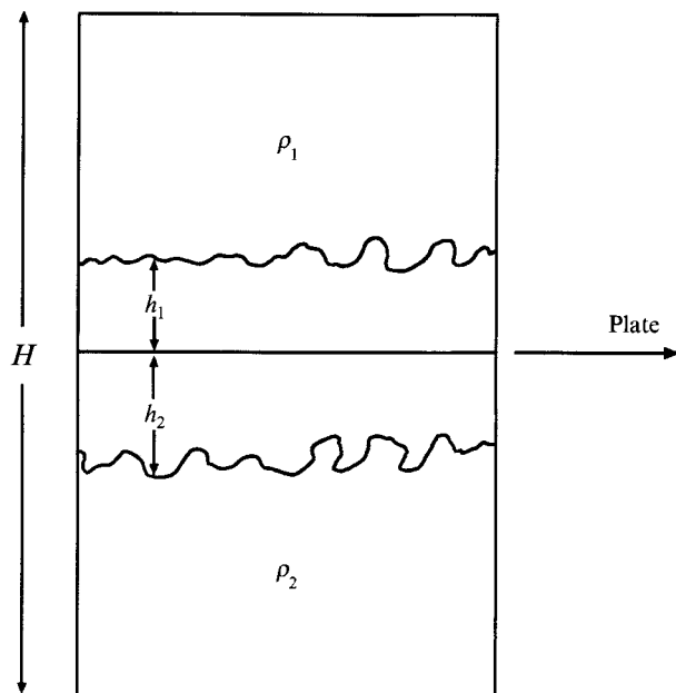
FIGURE 1. A sketch of the experimental configuration. The symbols are defined in the text.
